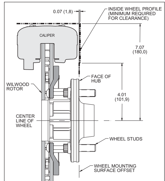
Figure 3. Wheel Clearance Diagram
